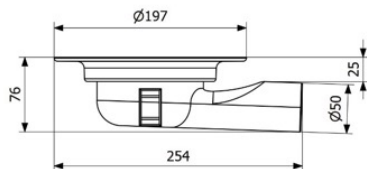
Siphon Compact Minimax (090G)
